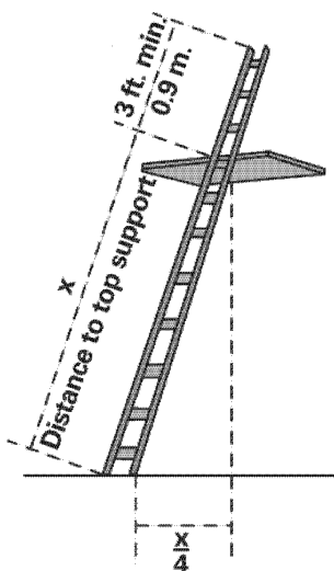
Figure D-1 -- Portable Ladder Set-up
