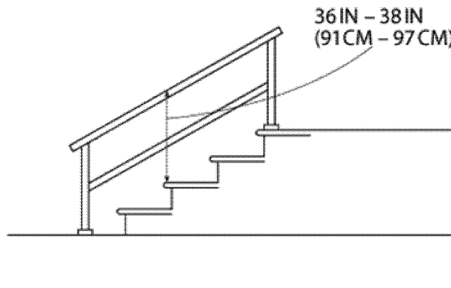
Figure D-13 – Combination Handrail and Stair Rail
