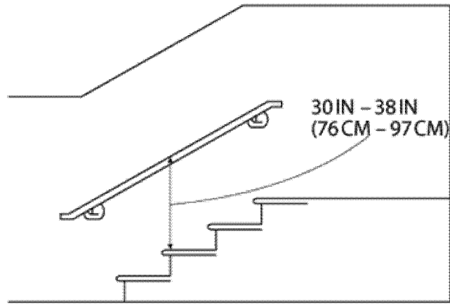
Figure D-12 – Handrail Measurement
